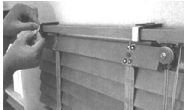
4 Fit the metal-clips and apply adhesive tape over the front of the clips
